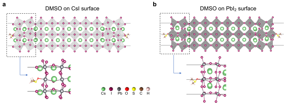
Figure S7 | Relaxed \text{CsPbI}_3 slabs with DMSO on a the \text{CsI} -terminated surface b the \text{PbI}_2 -terminated surface.
