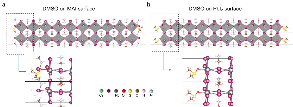
Figure S8 | Relaxed \text{MAPbI}_3 slabs with DMSO on a the \text{MAI} -terminated surface b the \text{PbI}_2 -terminated surface.
