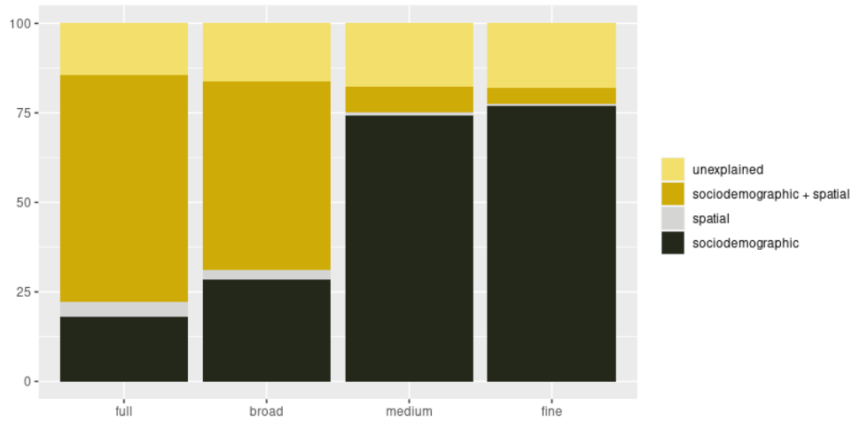
Figure 9: Variation partitioning
