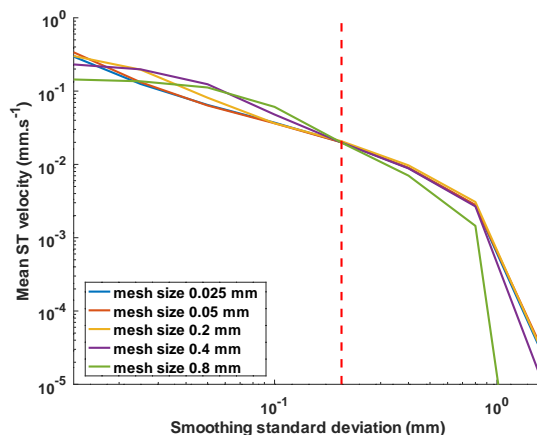
FIG. 4. Sensitivity of the mean Bingham fluid velocity (log-log) in the bifurcation relative to curvature smoothing (x-axis) and mesh refinement (colored curves). The finer the mesh, the more precise the quality of the finite elements method, but also the more sensitive the curvature is to the mesh. If the standard deviation of smoothing is too small, the fluid velocity is influenced by mesh specificities; conversely, if it is too large, the features of the bifurcation are lost. The chosen degree of smoothing is \sigma_d = 0.2 mm. A smaller value introduces artefacts due to the discretization into triangles of the bifurcation surface, while a larger value leads to over-smoothing, hiding the main geometrical features of the bifurcation. The chosen mesh size is 0.05 mm, corresponding to 186 594 triangles for meshing the bifurcation surface.
