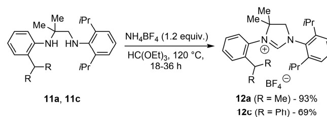
SCHEME 1 Synthesis of imidazolinium salts 12
