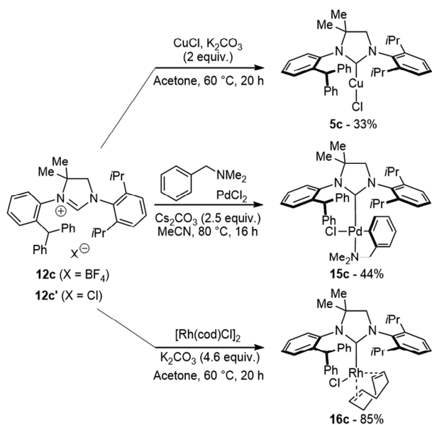
SCHEME 5 Synthesis of several metal complexes from imidazolium salt 12c
