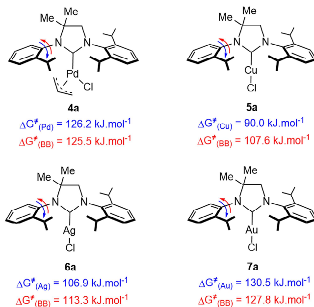
FIGURE 3 Determination of the rotational barrier values by DFT calculations (BB = backbone)
