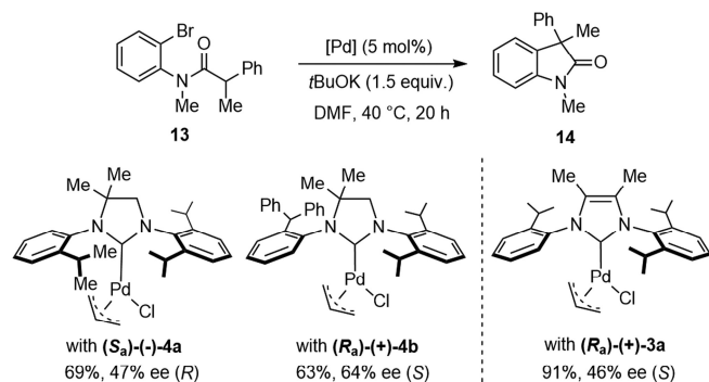
SCHEME 3 Intramolecular \alpha -arylation of amide 13 with NHC-palladium complexes 4
