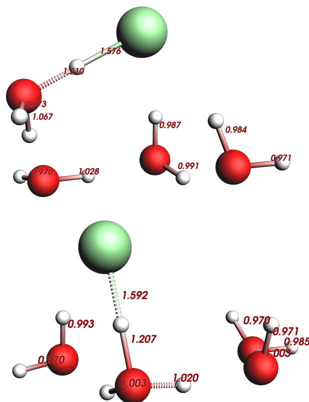
Fig. 7 Structures for a microsolvated HCl molecule originating from snapshots of model C, with nearest 4 waters shown. Internuclear distances (in Å) are indicated in the figure. Binding energies (in eV) for the [K, L 1 , L 2 , L 3 ] edges, obtained with CC-in-DFT (for the microsolvated system) are respectively [2832.6, 279.3, 208.7, 207.1] (Top) and [2831.9, 278.7, 208.0, 206.4] (Bottom).
