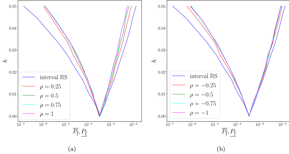
Figure 14: \mathbf{M}_2 comparison for positive coefficients of correlation (a) and \mathbf{M}_2 comparison for negative coefficients of correlation (b)
