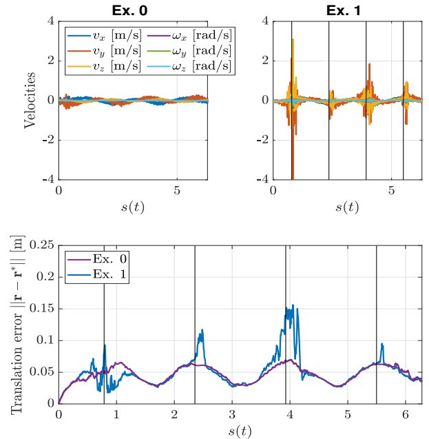
Fig. 13: Velocity inputs \tau_c (top) and translation error \|\mathbf{r} - \mathbf{r}^*\| during experiments 0 and 1. The vertical steps indicate where the trajectory in Ex. 1 traverses the singularity point \mathcal{P}_1 .
