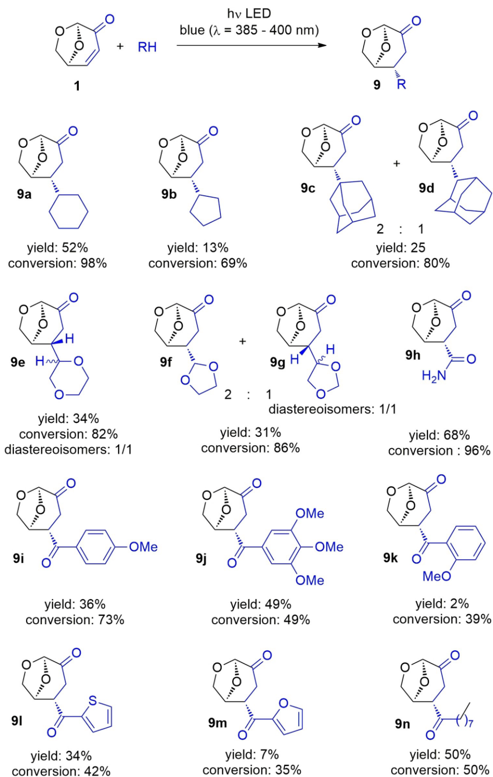
Scheme 4. Photocatalytical radical addition to levoglucosenone: blue LED, 5 equiv. RH, 5 mol% TBADT in MeCN (or MeCN/benzene: 70/30 in the case of 9c,d ), 8 h. Yields are given for isolated compounds.
