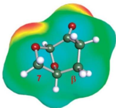
Figure 1. \sigma -Surface (COSMO surface) of dihydrolevoglucosenone (Cyrene) (with permission adapted from J. Sherwood, M. De bruyn, A. Constantinou, L. Moity, C. R. McElroy, T. J. Farmer, T. Duncan, W. Raverty, A. J. Hunt, J. H. Clark, Chem. Commun. 2014, 50, 9650–9652 (Copyright 2014) Royal Society of Chemistry).
