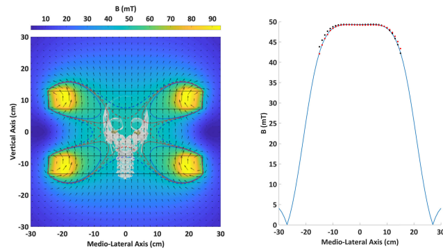
FIGURE 2. 2-D spatial illustration of the MF level distribution around the exposure system computed according to the Bio-Savart law (Left panel). The thick black rectangles represent the outer boundaries of both coils. Small black arrows represent the magnetic vector field. Red and blue lines represent respectively the boundaries of a 1% and 5% flux density variation limit area from the center. Dashed lines represent the lower boundary while solid lines represent the upper boundary. Participants' vestibular systems, illustrated by the yellow structures in the head, lie within a 50 mT ( \pm 0.5\% ) vertically- oriented homogeneous field. Flux density values for full head homogeneous ELF-MF stimulations targeted at 50 mT (right panel). The blue line represents the expected flux density values given by the model along the mediolateral axis. Red and black dots are actual flux density measurements along the mediolateral and anteroposterior axes respectfully.
