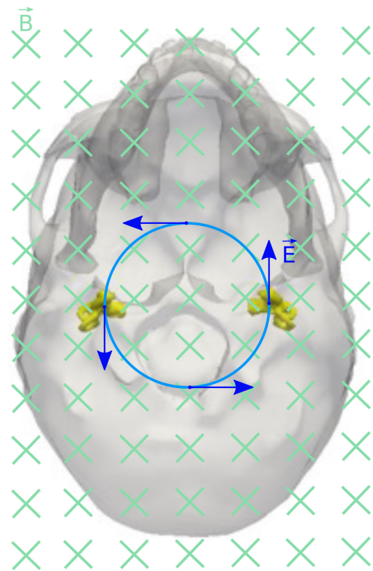
FIGURE 7. Bottom view of field orientation within a head representation. Both yellow structures are the vestibular systems. The green crosses represent the homogeneous MF increasing towards the top of the head. The light blue circle symbolizes a 5 cm radius Faraday's loop encompassing both vestibular systems. The dark blue arrows represent the tangential induced E-fields generated at selected points of the loop.
