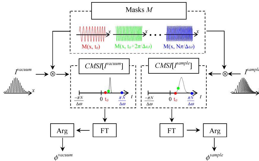
Fig. 2. Block diagram showing the procedure of extracting the spectral phases \phi^{\text{vacuum}} and \phi^{\text{sample}} from the channeled spectra I^{\text{vacuum}} and I^{\text{sample}} respectively. Masks M , CMSI[I^{\text{vacuum}}] and CMSI[I^{\text{sample}}] are complex quantities, only their amplitudes are represented in this diagram.
