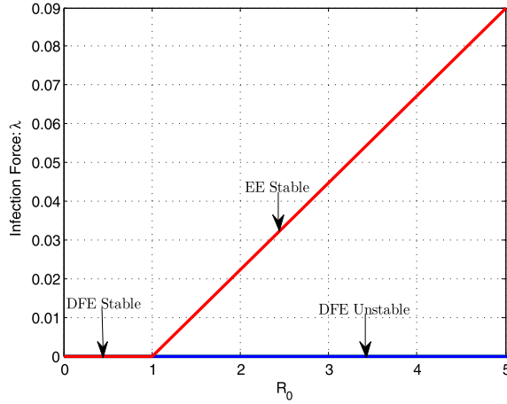
Fig. 2. Bifurcation diagram of model system (7). The notations DFE and EE stand for disease-free equilibrium and endemic equilibrium, respectively.
