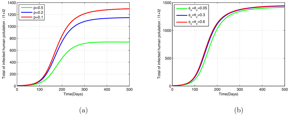
Fig. 5. Time series of the total number of infected individuals for three different values (a) the proportion of symptomatic infected individual \eta and (b) the virulence of bacteria \theta_v = \varphi_v .
