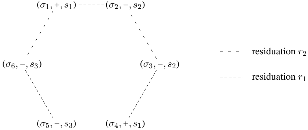
Figure 3: The 6 connectives of the orbit \mathcal{O}_{\alpha_2}((\sigma_1, +, s_1))
