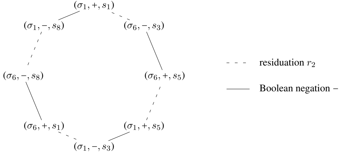
Figure 2: The 8 connectives of the orbit \mathcal{O}_{\alpha_{G_2}}((\sigma_1, +, s_1))
