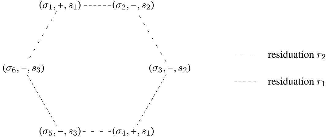
Figure 3: The 6 connectives of the orbit \mathcal{O}_{\alpha_2}((\sigma_1, +, s_1))
