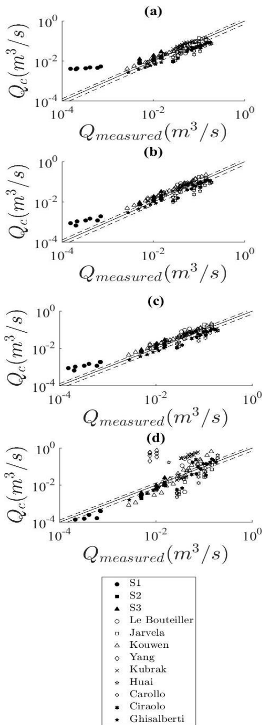
Fig. 6. Comparison of the total discharge over vegetated bed for the model of Huthoff (a), the Meijer and Van Velzen (b), Cassan and Laurens (c), and Rubol et al. (d) ( Cd = 1 for all experiments). Experiments from (Le Bouteiller and Venditti, 2015; Jarvela, 2005; Kouwen and Unny, 1969; Yang and Choi, 2009; Kubrak et al. , 2008; Huai et al. , 2009; Carollo, Ferro, Termini, 2002; Ciralo, Ferreri, 2007; Ghisalberti and Nepf, 2006). Dash lines represents a deviation of 30 %.
