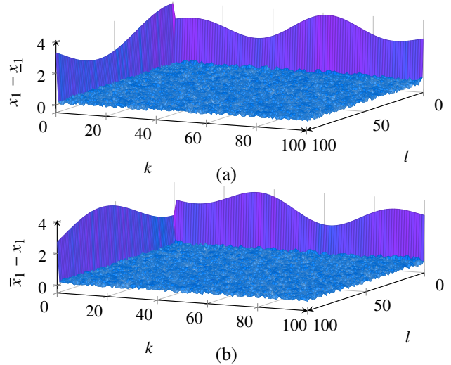
Fig. 3. Lower (a) and upper (b) estimation errors for the first state variable.
