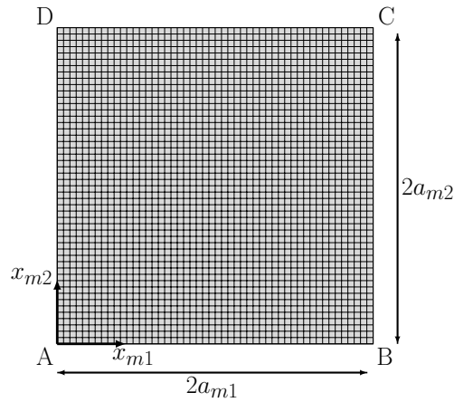
Figure 2: Finite element model of the representative volume element of the architected cellular material with its characteristic size for 2D problems.
