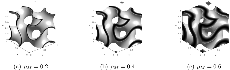
Figure 7: Examples of reconstruction of the T-Gyroid RVE topology for different values of relative density.
