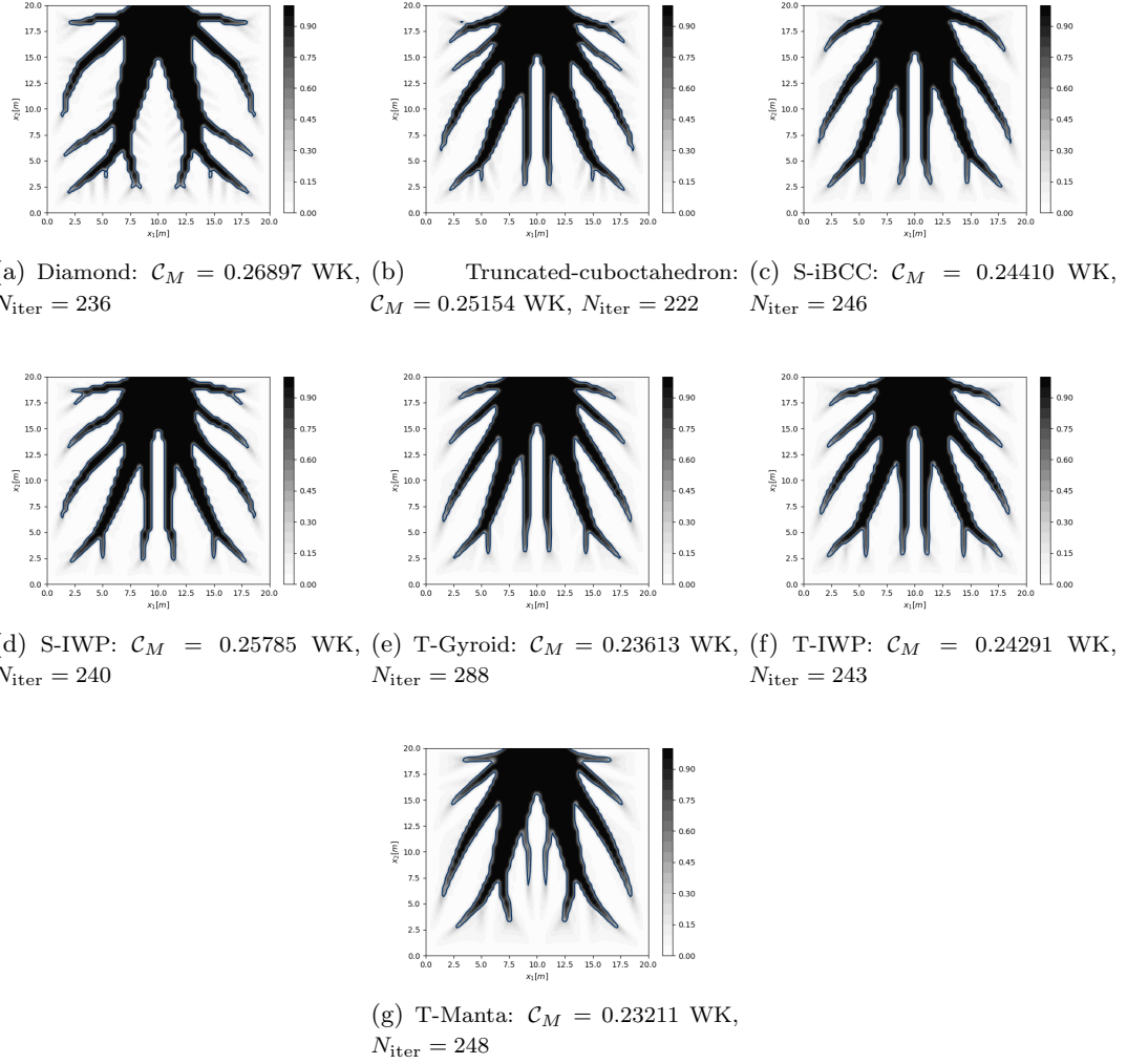
Figure 10: BK-2D: sensitivity of the optimised topology to the RVE geometry using B-spline entities with p_j = 2 ( j = 1, 2 ) and n_{MCP} = 68 \times 68 .
