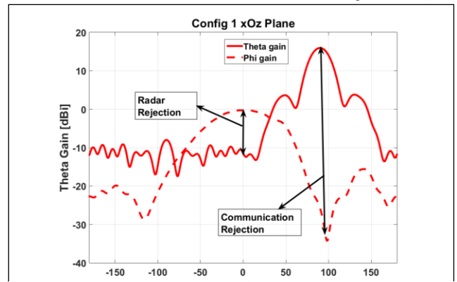
Figure 2: Radiation characteristics at 5 GHz
