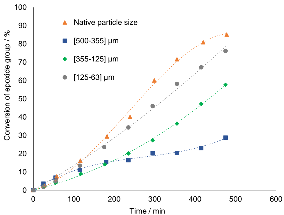
Fig.9. Effect of the particle size distribution of catalyst on the kinetics of carbonation reaction at 170 °C, 30 bar with [\text{EFAME}]_{\text{initial}} = 2.61\text{-}2.99 \text{ mol.L}^{-1} , catalyst loading = 0.32 \text{ mol.L}^{-1} and agitation speed of 500 rpm.
