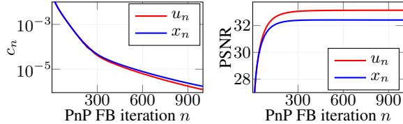
Fig. 2. Impact of the postprocessing along the iterations of Algorithm 8 on the BSD68 sample from Fig. 3.
