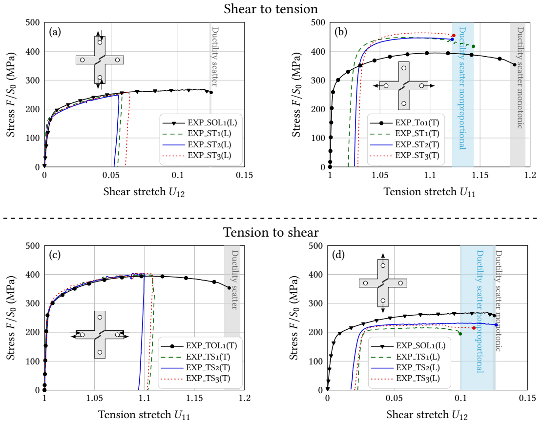
Figure 8 2198T3R non-proportional loading experimental results: (a) shear period and (b) tension period of ‘shear to tension’ (ST) loadings, (c) tension period and (d) shear period of ‘tension to shear’ (TS) loadings.
