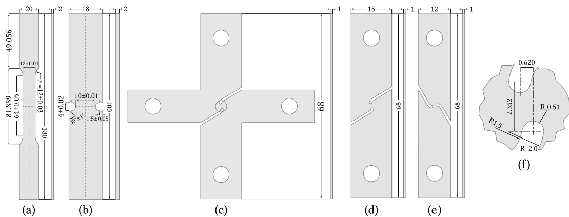
Figure 2 Macro specimen geometries with 2 mm thickness: (a) Uniaxial-tension (UT), (b) Notched-tension (NT2) and micro specimen geometries with 1 mm thickness: (c) Shear-tension cruciform for non-proportional loadings, (d) Shear-only (SO), (e) Tension-only (TO) samples and (f) the detailed geometry of the region of interest (ROI).
