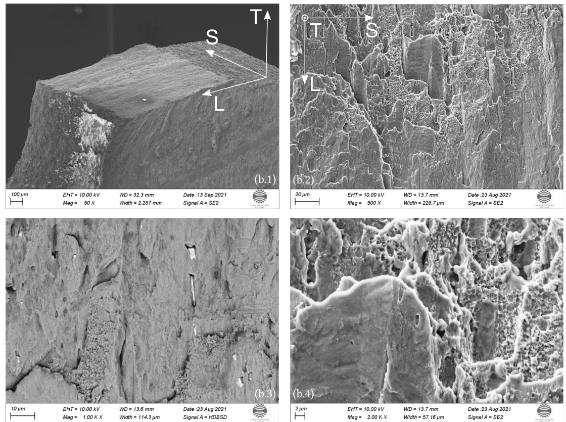
(b) Fractography under 'tension to shear' (TS): (b.1) Macroscopic smooth fracture surface, (b.2) shear fracture feature, (b.3) elongated intermetallic particles and (b.4) flat-like fracture feature with void sheeting features of submicro dimple cluster.
