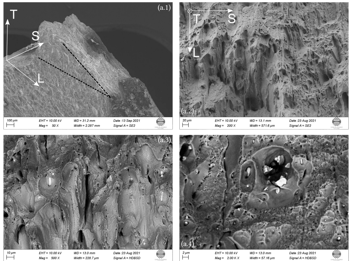
(a) Fractography under tension-only (TO): (a.1-2) Macroscopic rouge fracture surface with (a.3) large dimple that initiated to the intermetallic particles and (a.4) medium dimples with broken particles.
