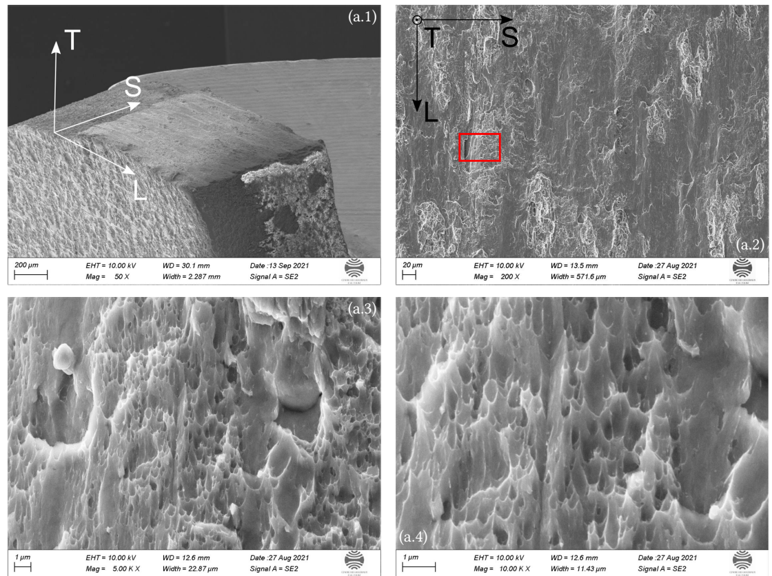
(a) Fractography under shear-only (SO): (a.1) Macroscopic smooth fracture surface, (a.2-3) flat fracture surface and (a.4) elongated ductile dimple cluster that initiated on the dispersoids.
