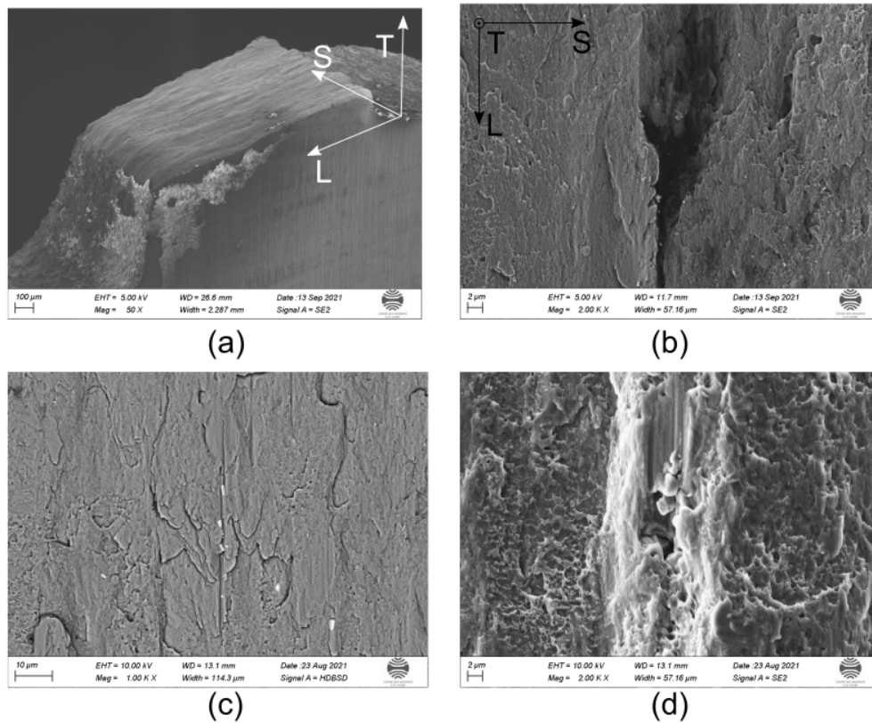
Figure 14: Fractography via scanning electron microscopy (SEM) of 2198T3R under ‘tension to shear’ (TS): (a) Macroscopic smooth fracture surface, (b) A flat crack-like feature is observed near middle thickness plane, (c) Intermetallic particles are elongated, broken and decohered, (d) Deformed intermetallic particles, medium dimples features including the void sheeting shear feature.
