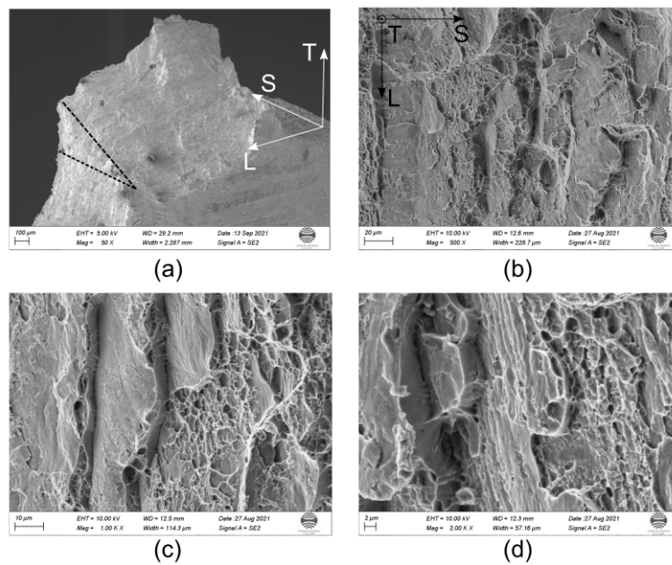
Figure 12: Fractography via scanning electron microscopy (SEM) of 2198T3R under 'shear to tension' (ST): (a) Macroscopic slant fracture path in T-S plane and relative smooth fracture surface, microscopic fracture features like (b) large dimples and (c)(d) grain-shaped steps with medium dimples.
