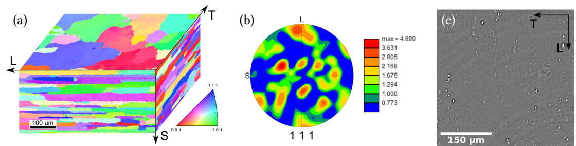
Figure 1 (a) Inverse pole figure indicating the 3D grain structure of 2198T 8 R sheet material via EBSD (the crystal orientations are given with respect to the normal of each plane), (b) Pole figure of 2198T 8 R and (c) 2D section of 2198T 8 R from high resolution 3D X-ray laminography in the L-T plane.
