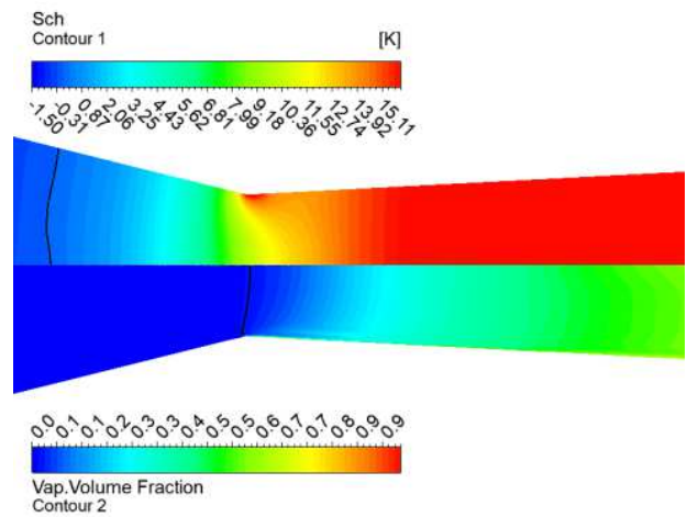
548 549 Figure 23 : Ohta B nozzle; 1.5K 100kPa; superheat and void fraction
