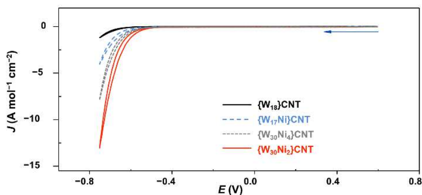
Figure 9. Comparison of the CVs obtained with POM/CNT hybrid materials deposited on a GC electrode. Current density, J , corrected with respect to the surface concentration of the hybrid deposited on the modified electrode. Electrolyte: 0.5 M H 2 SO 4 , pH = 0.3. Counter electrode: Pt; reference electrode: SCE. Scan rate: 2 mV s -1 .
