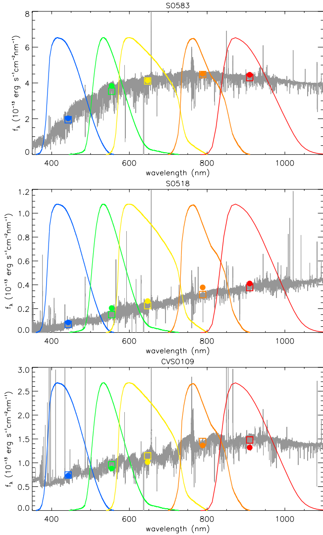
Fig. 2. X-shooter flux-calibrated spectrum of three of our targets (grey), as labelled, with quasi-simultaneous photometry for the same target obtained from OACT in the BVR_{CIZ}z' bands (dots). The filter bandpasses and the synthetic photometry (open squares) obtained integrating the spectrum over these bandpasses are overlaid.
