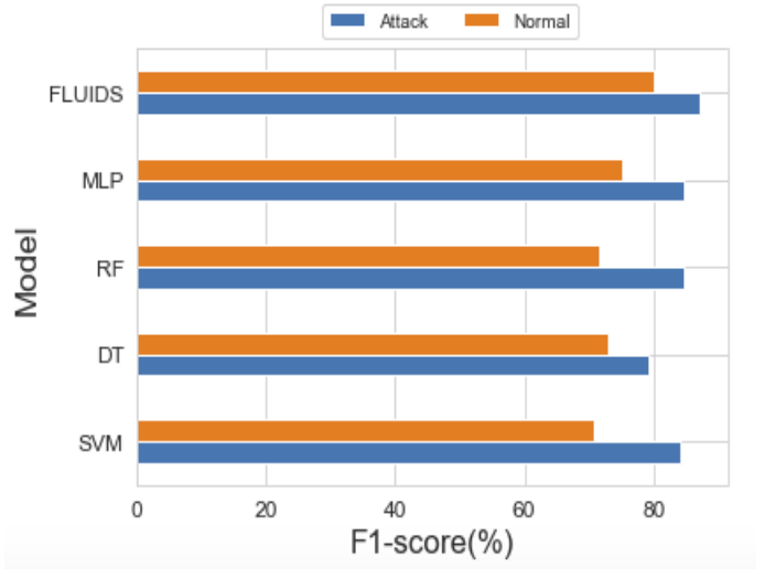
Figure 2. Comparison of FLUIDS performance to identify normal/attack IP flows against supervised models.
