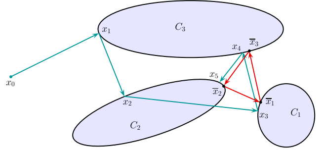
Fig. 6: The POCS algorithm with m = 3 sets and initialized at x_0 produces the cycle (\bar{x}_1, \bar{x}_2, \bar{x}_3) .
