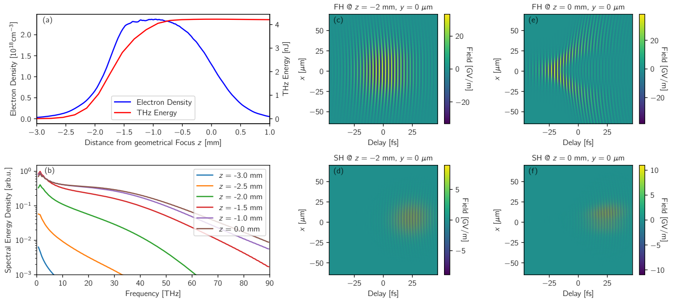
FIG. 5. THz source: (a) Peak plasma density and THz energy ( \nu < 90 THz) versus propagation distance relative to the geometrical focus at z = 0 . (b) Snapshots of the transverse integrated THz spectrum at several positions z along the plasma. Snapshots of the main FH (c) and SH (d) polarization component of the pump field near the beginning of the plasma at z = -2 mm. (e) and (f) show the same fields near the end of the plasma at the geometrical focus z = 0 .
