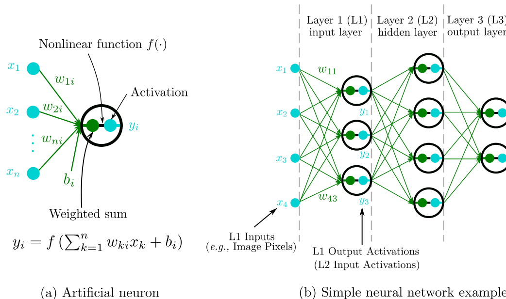
Figure 1: A basic DNN example and the associated terminology (adapted from [SCYE20, Figure 1.3]).
