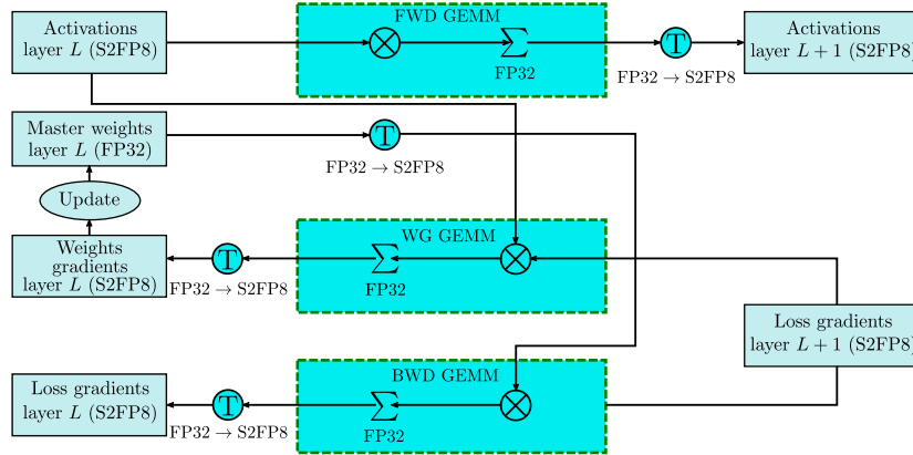
Figure 14: The low precision training flow with the S2FP8 format, where the truncation function T corresponds to T(X) = \left[2^{-\beta} \left\{\text{round}_{\text{FP8}}(2^{\beta}|X|^{\alpha})\right\}\right]^{1/\alpha} . The forward and backward GEMM operations use only S2FP8 values, whereas the weight update step uses FP32 master weights (adapted from [CBG + 20, Fig. 4]).
