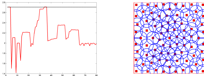
Figure 2: Designs generated by \mathbf{x}_{n+1} \in \text{Arg max}_{\mathbf{x} \in \mathcal{X}} D_4(\mathbf{x}, \mathbf{X}_n, \mathcal{X}) in \mathcal{X} = [0, 1]^2 with \|\cdot\| = \|\cdot\|_2 and \mathbf{x}_1 = (1/2, 1/2) . Left: \text{MR}(\mathbf{X}_n) for n = 2, \dots, 80 ; the horizontal line indicates the upper bound 2(1 + \sqrt{d}/\beta) on \text{MR}(\mathbf{X}_n) . Right: \mathbf{X}_{80} ; the circles have radii h(\mathbf{X}_n) = 0.0913 .
