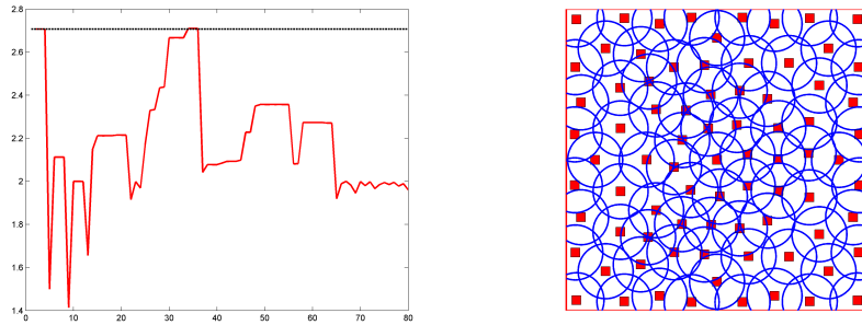
Figure 2: Designs generated by \mathbf{x}_{n+1} \in \text{Argmax}_{\mathbf{x} \in \mathcal{X}} D_4(\mathbf{x}, \mathbf{X}_n, \mathcal{X}) in \mathcal{X} = [0, 1]^2 with \|\cdot\| = \|\cdot\|_2 and \mathbf{x}_1 = (1/2, 1/2) . Left: \text{MR}(\mathbf{X}_n) for n = 2, \dots, 80 ; the horizontal line indicates the upper bound 2(1 + \sqrt{d}/\beta) on \text{MR}(\mathbf{X}_n) . Right: \mathbf{X}_{80} ; the circles have radii h(\mathbf{X}_n) = 0.0913 .
