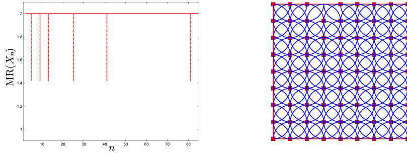
Figure 1: Designs generated by Algorithm 1 in \mathcal{X} = [0, 1]^2 with \|\cdot\| = \|\cdot\|_2 and \mathbf{x}_1 = (1/2, 1/2) . Left: \text{MR}(\mathbf{X}_n) for n = 2, \dots, 85 . Right: \mathbf{X}_{80} ; the circles have radii h(\mathbf{X}_{80}) = \gamma_2/2 = 0.125 .
