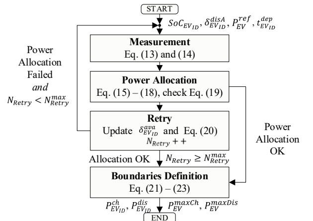
Fig. 2: Summary of the EVPA module algorithm
