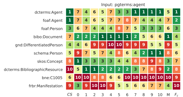
Figure 12: Rankings for entity type in the Gutenberg dataset.
