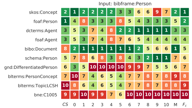
Figure 11: Rankings for entity type in the University dataset.
