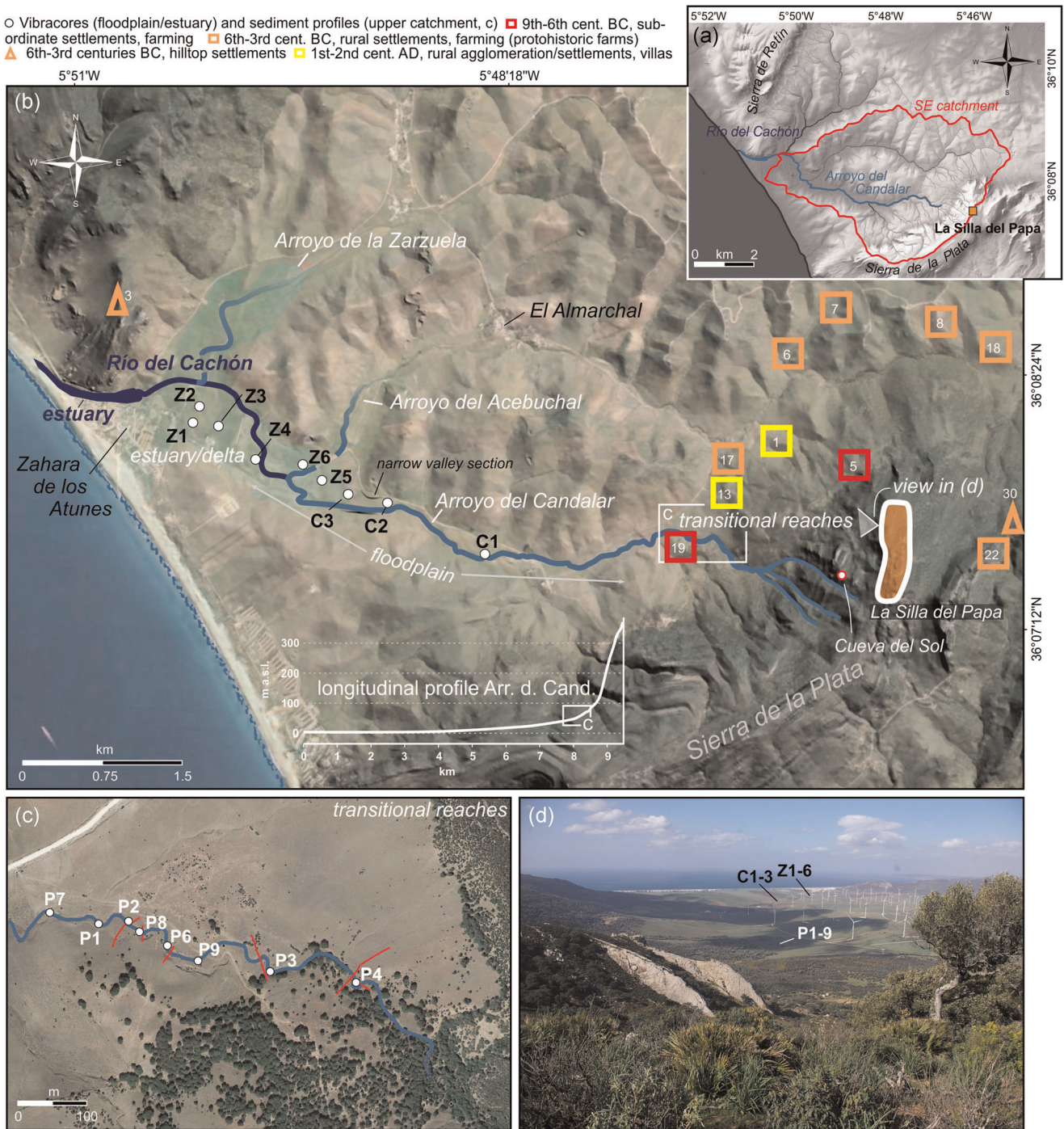
FIGURE 2 Setting and overview of the study area. (a) The catchment of the Río del Cachón, debouching into the Atlantic Ocean close to Zahara de los Atunes; boundary of the Arroyos del Candalar and del Acebuchal sub-catchment is marked by red line (“SE catchment”). (b) Overview of the catchment of the Arroyo del Candalar, including locations of sediment cores in the lower floodplain and relevant archaeological remains (based on Jiménez-Vialás & Grau-Mira, 2019; numbers of archaeological sites refer to the same reference). La Silla del Papa is located just above the upper reaches of the Arroyo. Noted is also the longitudinal profile of the Arroyo del Candalar. (c) Upper catchment area with locations of sediment profiles P1 to P9. (d) Overview of the study area (i.e., the low-relief coastal area east of Zahara de los Atunes) from La Silla del Papa; view towards west, Atlantic Ocean in the background. Red lines = topographical transects where terrace levels were documented [Color figure can be viewed at wileyonlinelibrary.com ]
