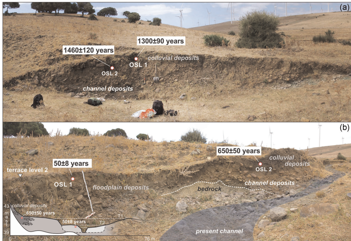
FIGURE 5 Sediment profiles P6 (a) and P8 (b) with OSL ages from colluvial and alluvial units, documented along undercut slopes of the incised river bed. Terrace level 1 is not visible in the photos but is indicated in the schematic sketch shown in (b) [Color figure can be viewed at wileyonlinelibrary.com ]
