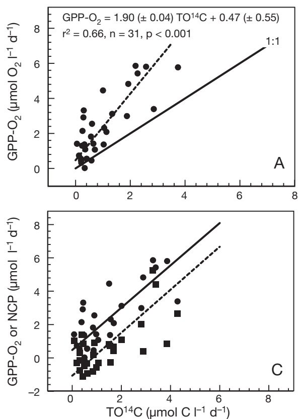
Fig. 3. (A) Relationship between gross primary production measured by the light-dark O_2 method ( GPP-O_2 ) and daily ^{14}C uptake. (B) Relationship between net community production (NCP) measured by the light-dark O_2 method and daily ^{14}C uptake. Dashed lines = reduced major axis (RMA) regressions. (C) Relationship between TO^{14}C and NCP (dashed line and circles; 1.14 \pm 0.08 \times TO^{14}C - 1.07 \pm 0.64 ), and GPP-O_2 (solid line and squares; 1.19 \pm 0.04 \times TO^{14}C + 0.47 \pm 0.55 ), assuming a photosynthetic quotient of 1.5
