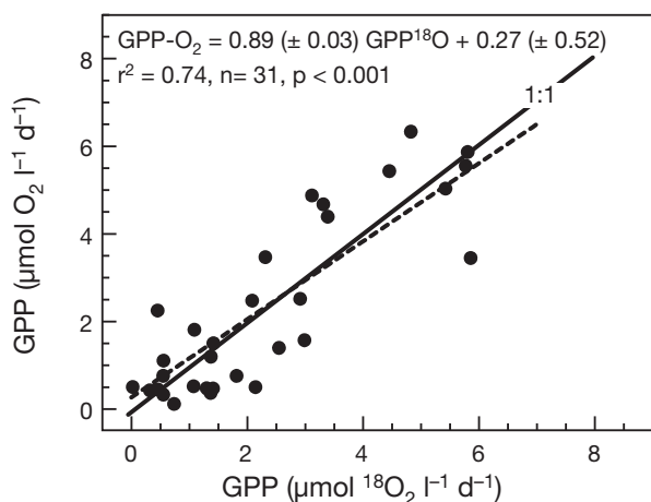
Fig. 2. Relationship between gross primary production measured by the light-dark O_2 method ( GPP-O_2 ) and gross primary production measured by the ^{18}O technique ( GPP-^{18}O ).
