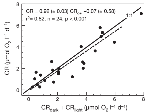
Fig. 1. Relationship between community respiration ( \text{CR}_{\text{dark}} + \text{CR}_{\text{light}} [ \text{CR}_{\text{d+1}} ] estimated as the sum of dark and light respiration rates and community respiration (CR) estimated from the light–dark O_2 method. Dashed line = reduced major axis (RMA) regression
