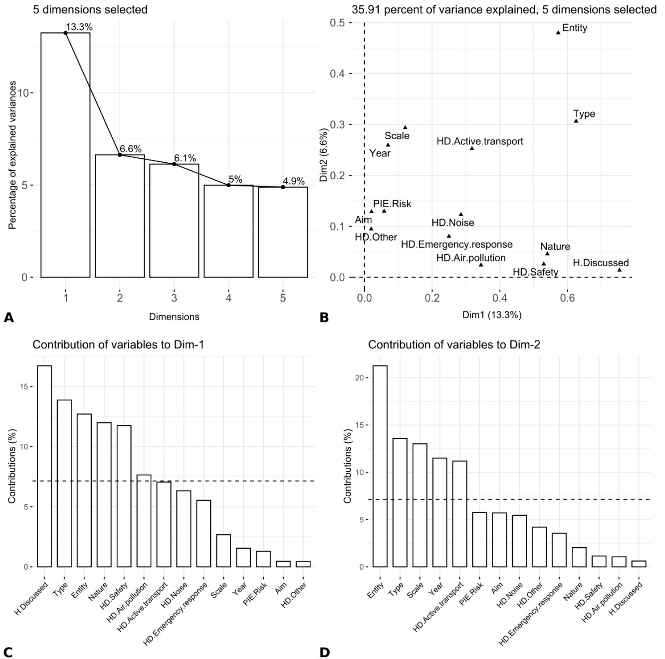
Figure 1. Factor Analysis of Mixed Data: contribution of the variables explaining the most the variation of the dataset. (A) 5 dimensions scree plot showing the percentage of explained variation per dimension. (B) The plot of variables from dimensions 1 and 2. (C) Contribution of variables to dimension 1. The dashed line shows the expected average value if the contributions were uniform. (D) Contribution of variables to dimension 2. The dashed line shows the expected average value if the contributions were uniform. HD for 'Health Discussed'.
