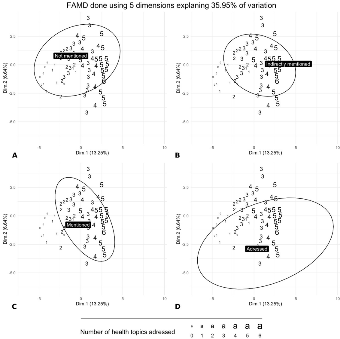
Figure 2. Factor Analysis of Mixed Data: representation of the first two dimensions, in terms of how the EPI risk was discussed, based on the number of health topics addressed.
