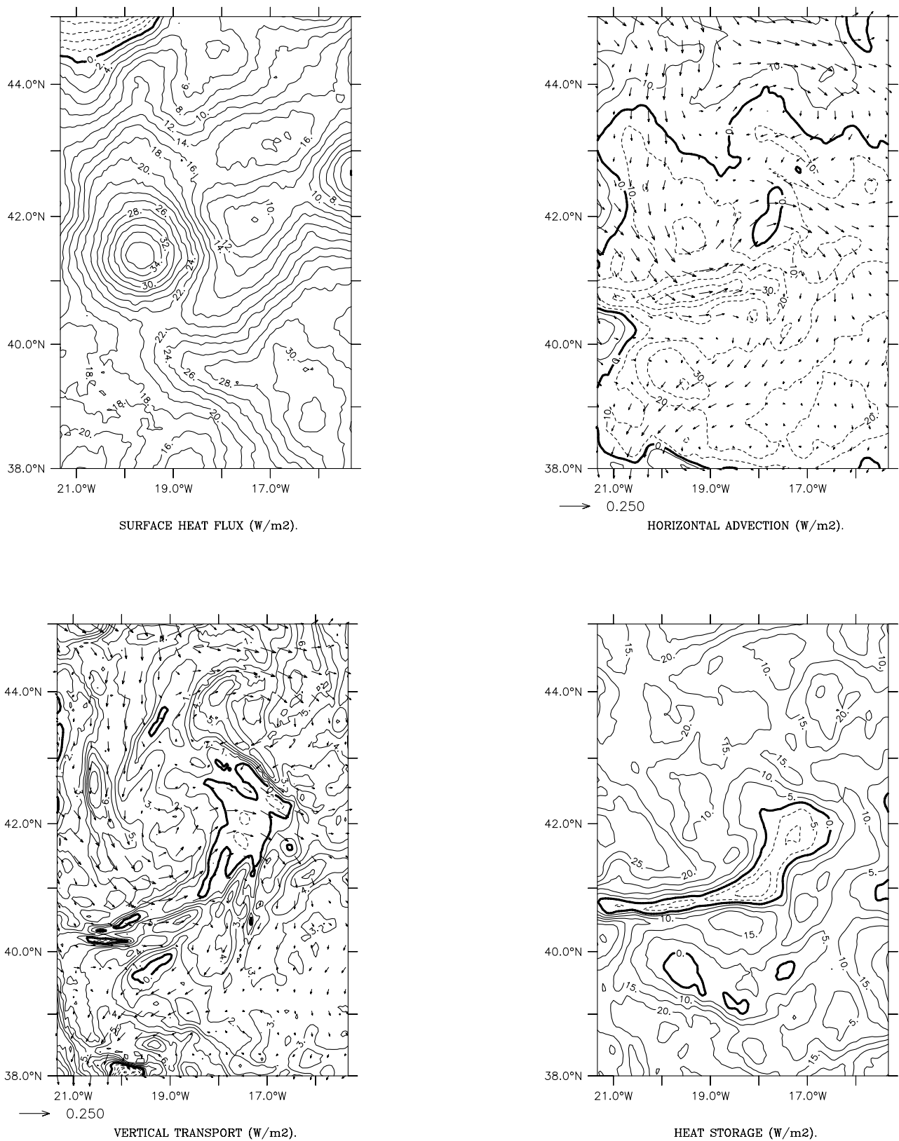
Figure 12. Annual mean charts of each term of the mixed layer heat budget. Units are in W m^{-2} , obtained by dividing each term of the mixed layer heat budget by the total cumulative time (343 days). The annual mean surface current ( m s^{-1} ) is superimposed onto the horizontal advection and vertical heat transport. Contour intervals are 2 W m^{-2} for surface heat flux; 10 W m^{-2} for horizontal advection; 1 W m^{-2} for vertical transport; and 5 W m^{-2} for the mixed layer heat budget.
