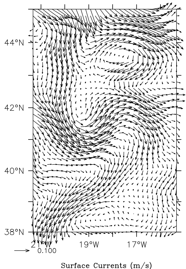
Figure 4. Annual averaged simulated surface currents.
