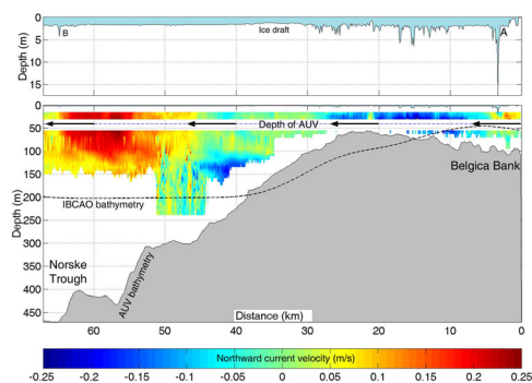
Figure 2. The outward track of mission 365, 21–22 August 2004, runs at 40 m depth. (top) Ice draft measured at crude resolution by upward-looking ADCP; A and B are ridges shown in Figure 3 whose depths are underestimated by the ADCP. Note smooth undeformed ice over Norske Trough. (bottom) The seabed topography measured by Autosub compared with the IBCAO bathymetry (dashed line). The coloured masses are N-S velocity components measured by the downward looking ADCP aboard Autosub. The red area is a strong northward current in the Trough, the Northeast Greenland Coastal Current (NGCC); the blue area is a hitherto unrecognised southward current on the western flank of Belgica Bank.
