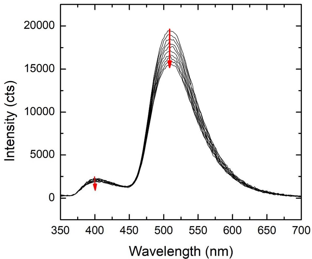
Figure 5. Fluorescence spectra ( \lambda_{\text{exc}} = 320 \text{ nm} ) of freshly-prepared 3HF-doped MCM-41 NPs after different period of UV light ( \lambda = 320 \text{ nm} ) exposure. Spectra were recorded every 3 minutes. Intensity (for both emission bands) decreases with time, as indicated by the red arrows.
