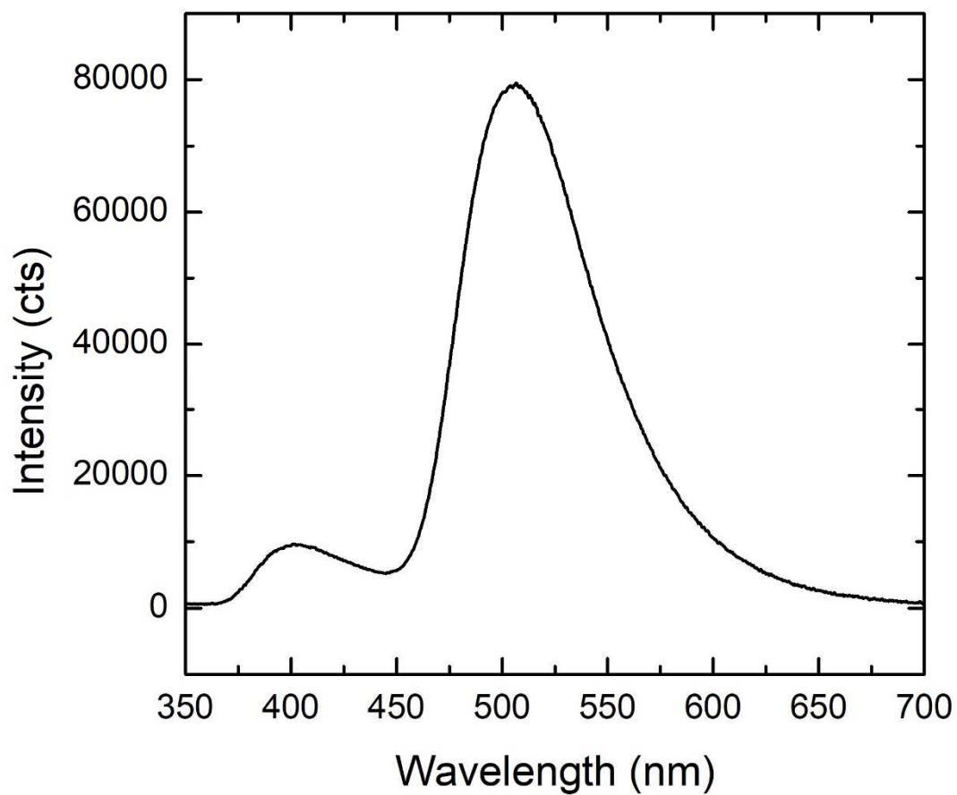
Figure 3. Fluorescence spectrum ( \lambda_{\text{exc}} = 320 \text{ nm} ) of aged (2 months of air exposure at 298K) 3HF-doped MCM-41 NPs. The fluorescence spectrum of freshly-prepared 3HF-doped MCM-41 NPs is shown in Fig. 3 of the related research paper [6].
