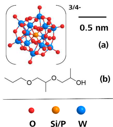
Fig. 1. (a) Representative structure of \alpha -Keggin-type polyoxometalate anion ( i.e. PW_{12}O_{40}^{3-} (PW), SiW_{12}O_{40}^{4-} (SiW)) and (b) an isomer of C_3P_2 . Note, that in the present study only the acidic forms of the POMs, i.e. H_3PW_{12}O_{40} and H_4SiW_{12}O_{40} , are considered.
