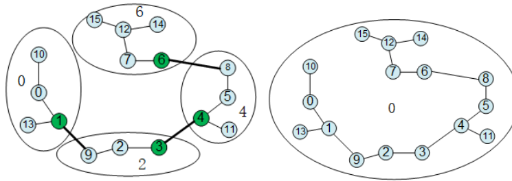
(c) Connect Graph : Add link to each winner node's and to its correspondent node's (green) adjacency list .
