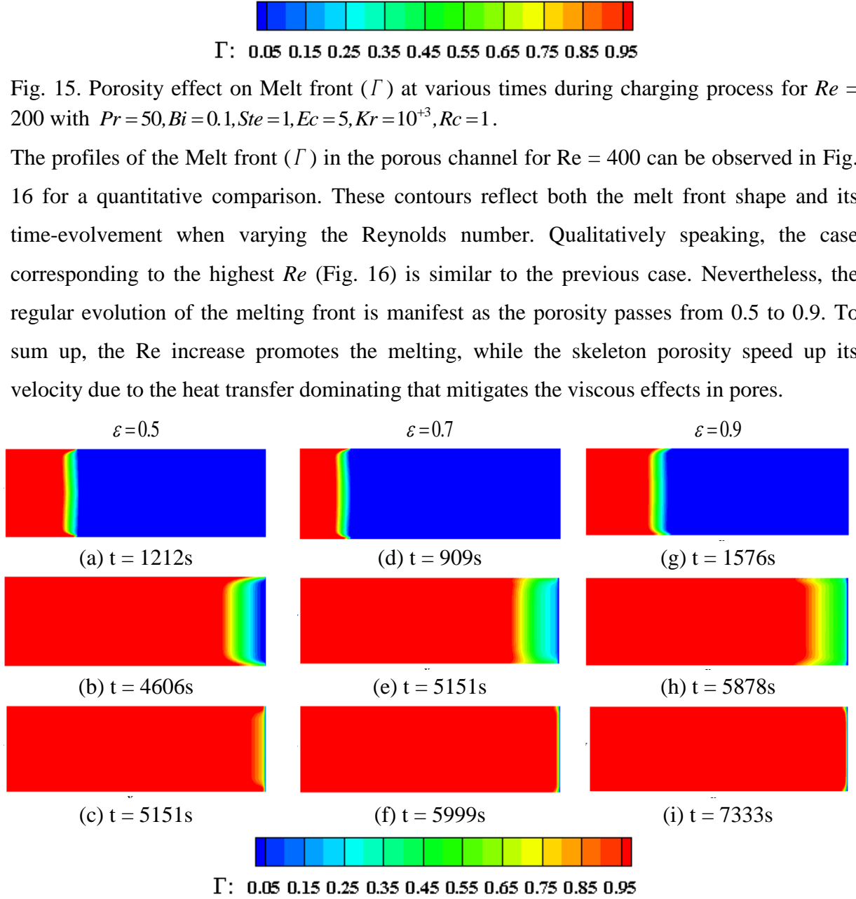
Fig. 16. Porosity effect on Melt front ( \Gamma ) at various times during charging process for Re = 400 with Pr = 50, Bi = 0.1, Ste = 1, Ec = 5, Kr = 10^{+3}, Rc = 1 .
