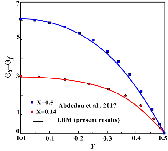
Fig. 6. LTNE intensity ( \Theta_s - \Theta_f ) vs. dimensionless distance Y at two axial positions for Da = 10^{-4}, Bi = 10^{-2}, Re = 10^2 = Rq and Kr = 1 .
