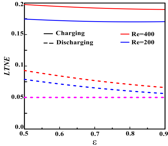
Fig. 8. LTNE parameter during charging and discharging vs. \varepsilon parameterized by Re , and at Pr = 50, Bi = 0.1, Ste = 1, Kr = 10^{+3}, Ec = 5, Rc = 1 . Also plotted in the figure is the LTNE's minimum value (5%) commonly accepted (the horizontal dotted line).
