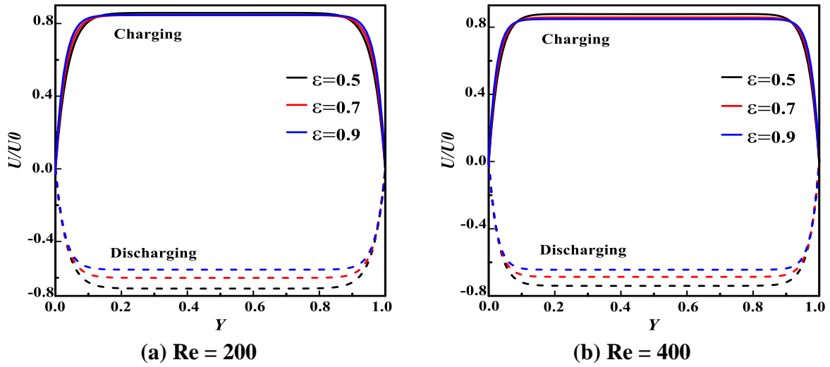
Fig. 9. Porosity effect on U-velocity during charging and discharging processes for two Re numbers at X = 0.5 with Pr = 50, Bi = 0.1, Ste = 1, Kr = 10^{+3}, Ec = 5, Rc = 1 .
