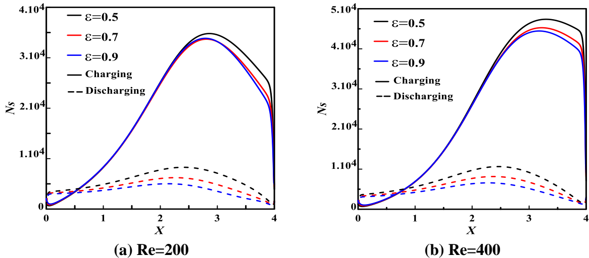
Fig. 11. Porosity effect on the entropy generation rate ( Ns ) during charging and discharging processes for two Re numbers at Y = 0.5 with Pr = 50, Bi = 0.1, Ste = 1, Kr = 10^{+3}, Ec = 5, Rc = 1 .
