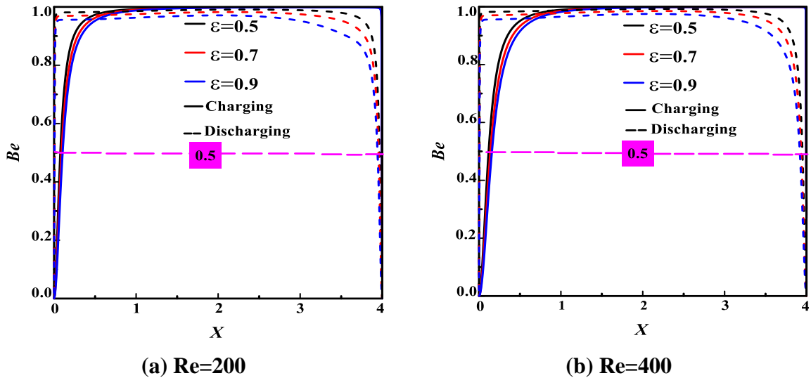
Fig. 13. Porosity effect on the Bejan number ( Be ) during charging and discharging processes for two Reynolds numbers at Y = 0.5 with Pr = 50, Bi = 0.1, Ste = 1, Kr = 10^{+3}, Ec = 5, Rc = 1 .
