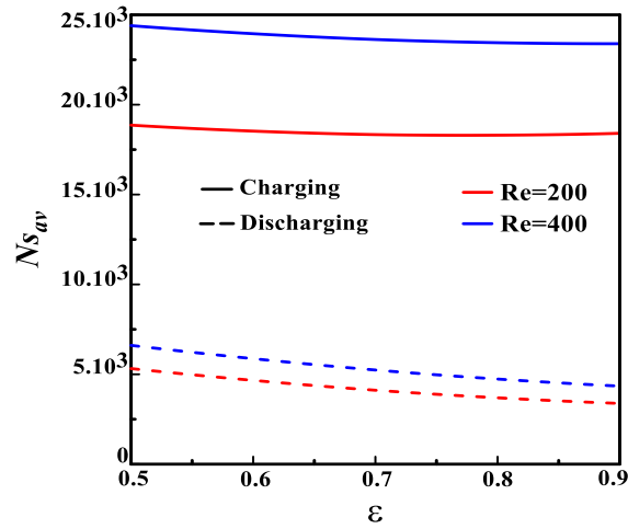
Fig. 12. Porosity effect on the average entropy generation rate ( N_{s_{av}} ) during charging and discharging processes for two Re numbers with Pr = 50, Bi = 0.1, Ste = 1, Kr = 10^{+3}, Ec = 5, Rc = 1 .
