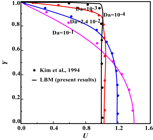
Fig. 5. Darcy number's effect on velocity profiles vs. dimensionless transverse distance at X = 0.5 for Re = 50 and Pr = 0.7 .
