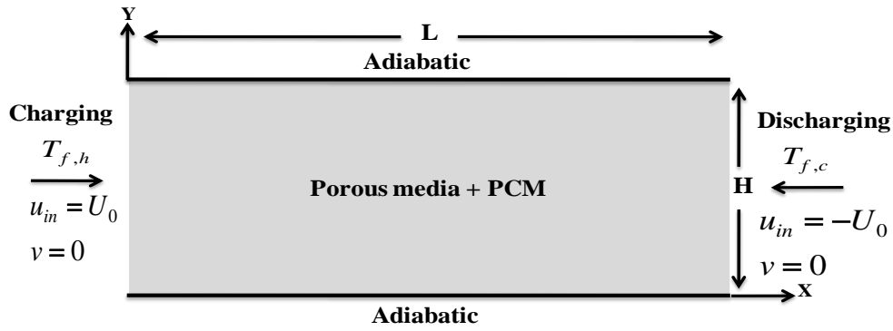
Fig. 1. Schematic view of the physical model along with boundary conditions (charging and discharging cases).
