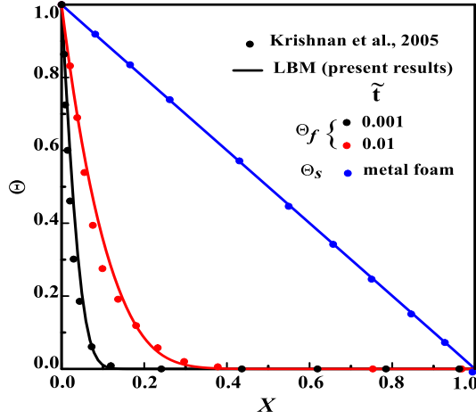
Fig. 7. Dimensionless fluid and solid temperature evolution ( \Theta_f, \Theta_s ) vs. dimensionless transverse distance X at Y = 0.5 for a nil interstitial Nusselt ( Nu_i = 0 ) and Da = 10^{-2}, Pr = 50, Ra = 10^6, Ste = 1 .
