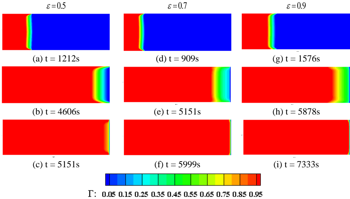
Fig. 16. Porosity effect on Melt front ( \Gamma ) at various times during charging process for Re = 400 with Pr = 50, Bi = 0.1, Ste = 1, Ec = 5, Kr = 10^{+3}, Rc = 1 .
