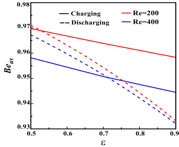
Fig. 14. Porosity effect on the average Bejan number ( Be_{av} ) during charging and discharging processes for two Reynolds numbers with Pr = 50, Bi = 0.1, Ste = 1, Ec = 5, Kr = 10^{+3}, Rc = 1 .
