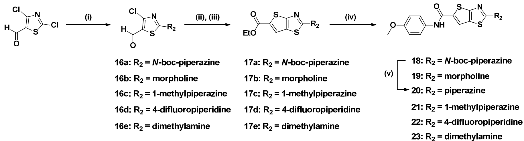
Scheme 2. Scheme for the synthesis of TTCA derivatives 18-23.
