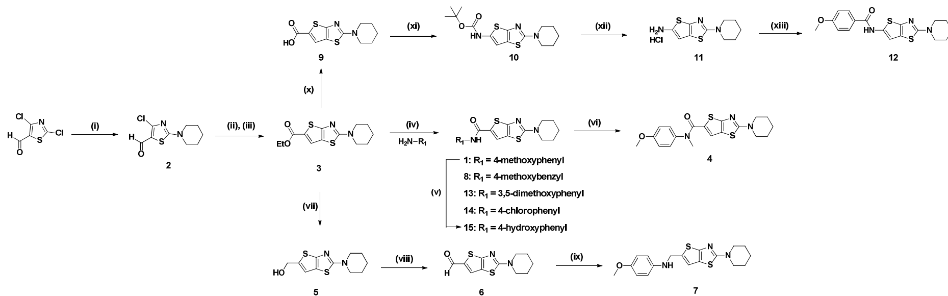
Scheme 1. Scheme for the synthesis of TTCA analogues with modified linkers.
