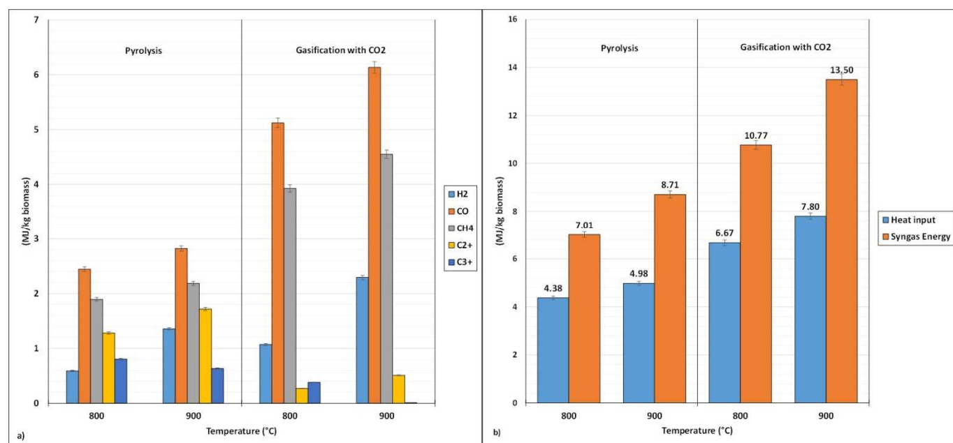
Figure. 6 Comparison between pyrolysis and gasification; Agent CO 2 /N 2 , bed material: sand a) energy distribution for gases and b) heat input Vs Syngas Energy.
