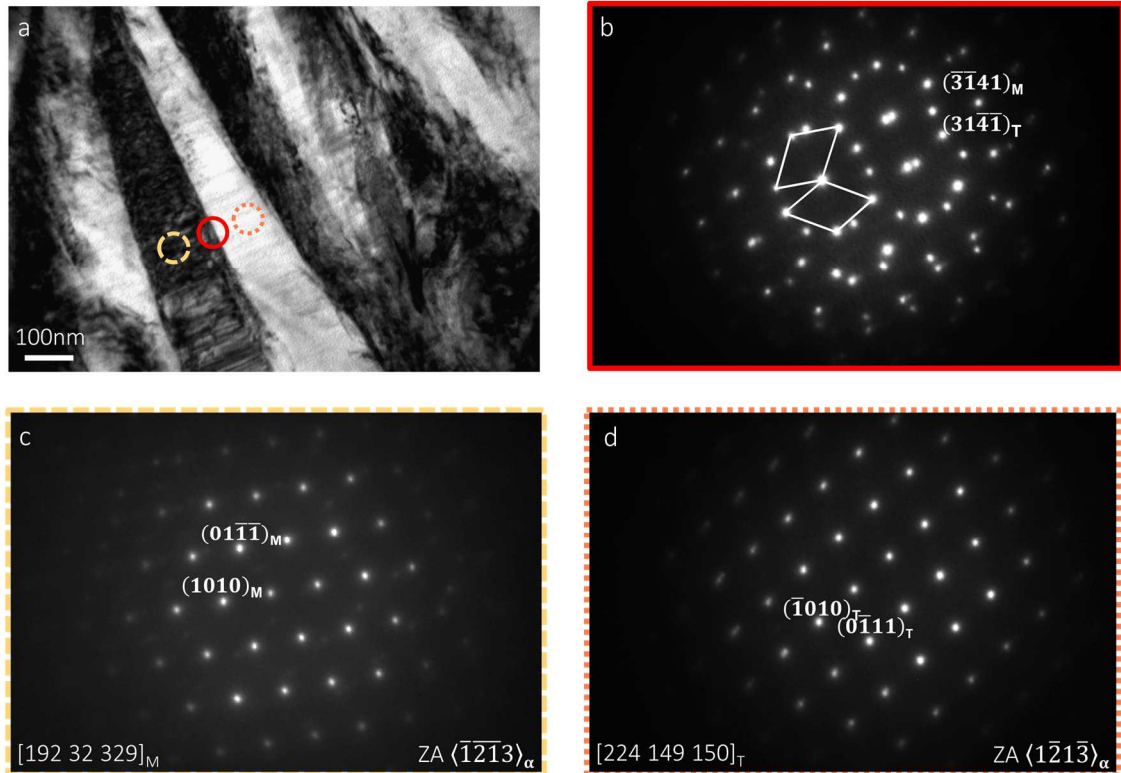
Fig. 4 a : Bright field micrograph of 2 parallel martensite plates, b : SAED pattern of the area encircled in red in Fig. 4a, c : SAED pattern of the area encircled in yellow (lath in dark of the left on the studied interface) in Fig. 4a, d : SAED pattern of the area encircled in orange (bright lath on the right on the studied interface) in Fig. 4a.
