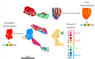
\alpha' martensite variants after deformation
