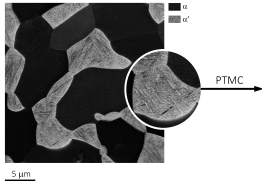
\alpha' + \alpha dual-phase microstructure
