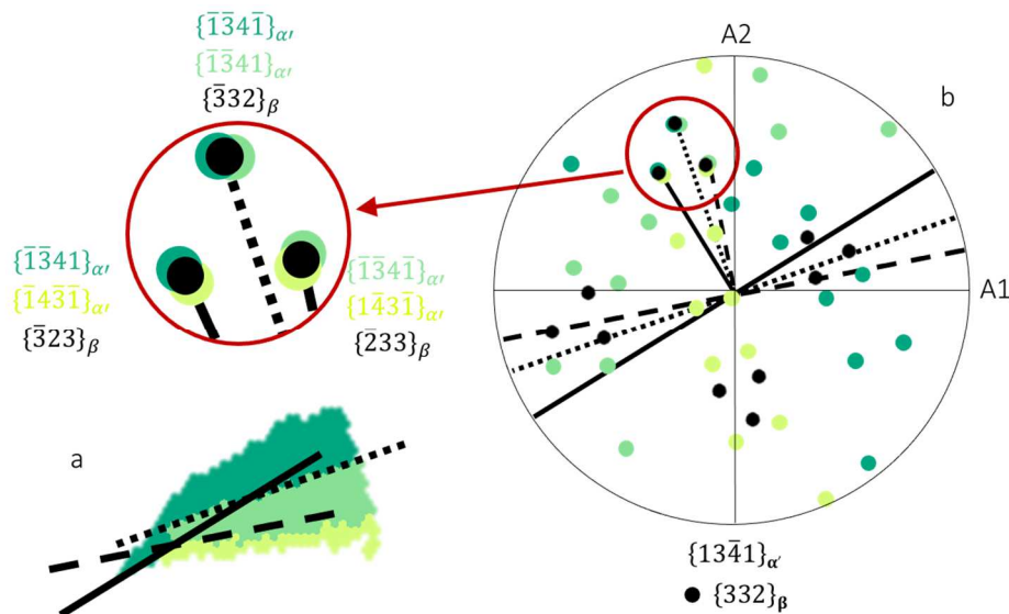
Fig. 5 a : IPF map of the variants formed in grain 2 of Fig. 3. ; b : \{13\bar{4}1\}_{\alpha'} stereographic projections of the 12 possible variants that could form in grain 2 superimposed onto the \{332\}_{\beta} pole figure of the parent \beta grain.
